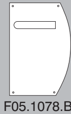
30mm lever on 3mm thick laser-cut latchplate
