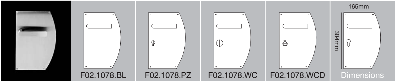
25mm lever on 3mm thick laser-cut latchplate
