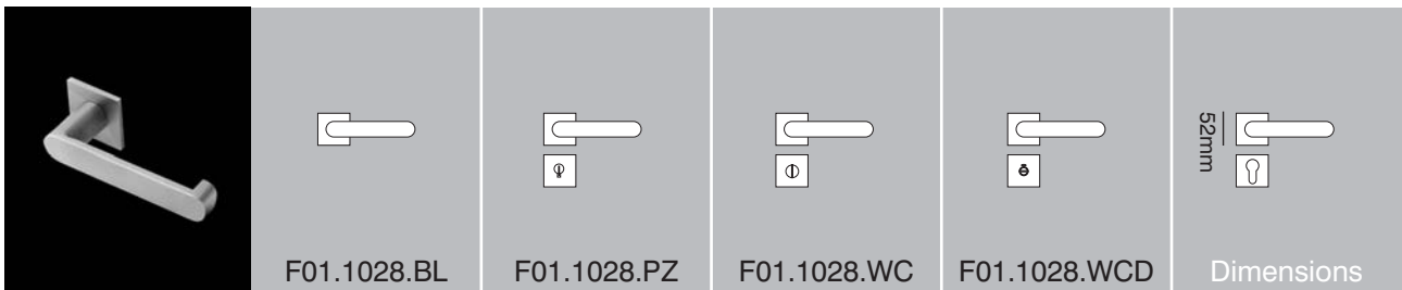
25mm lever on 52 x 52 x 4mm square concealed fixing rose
