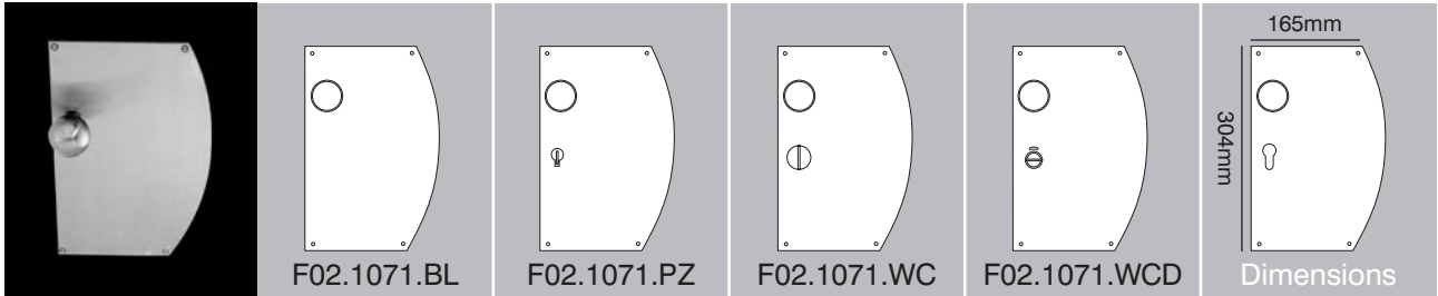
52mm dia knob on 3mm thick laser-cut latchplate
