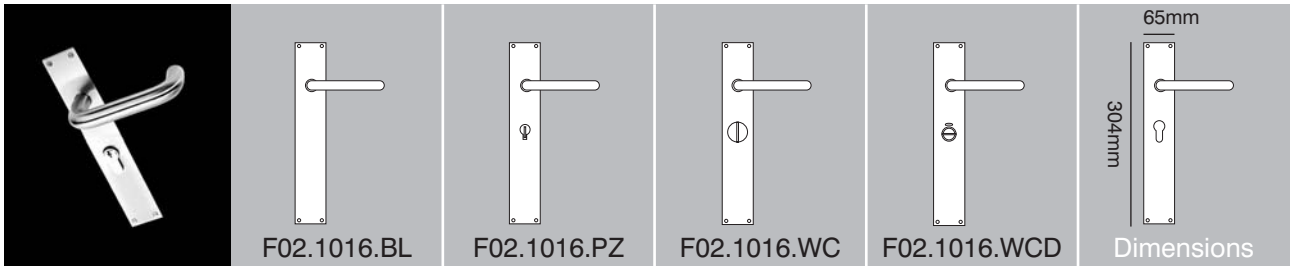
19mm lever on 3mm thick laser-cut euro backplate
